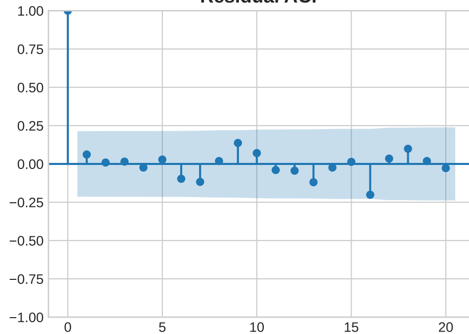
Residual ACF
