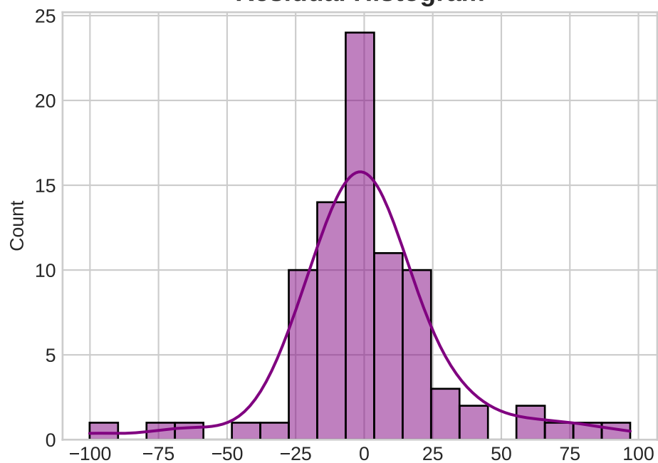
Residual Histogram
