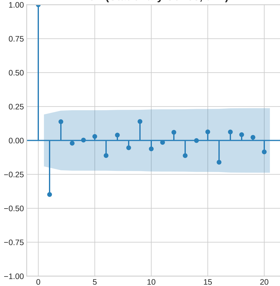
ACF (Stationary Series, d=1)
