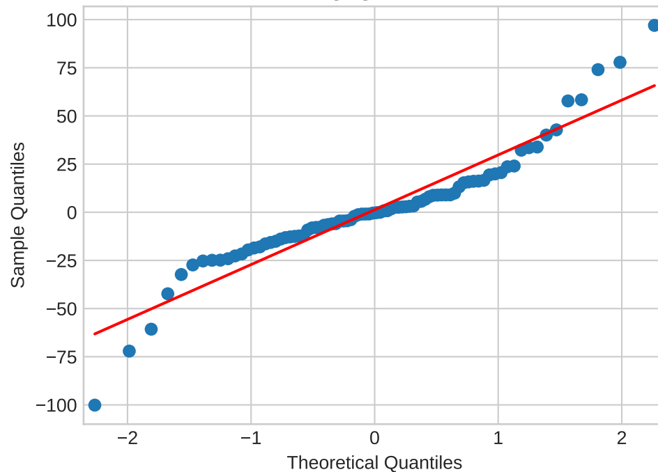
Q-Q Plot
