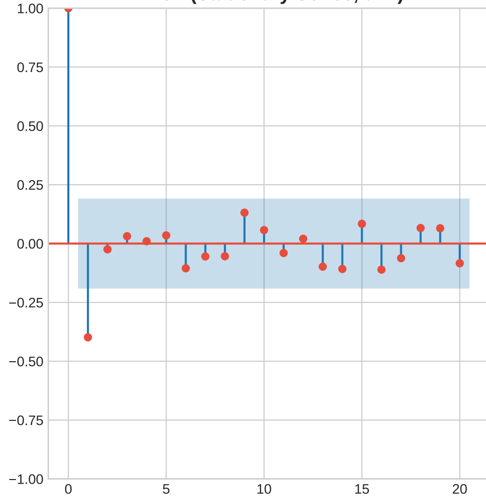
PACF (Stationary Series, d=1)
