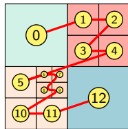
Z-Order Traversal
