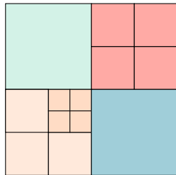
2D AMR Mesh
