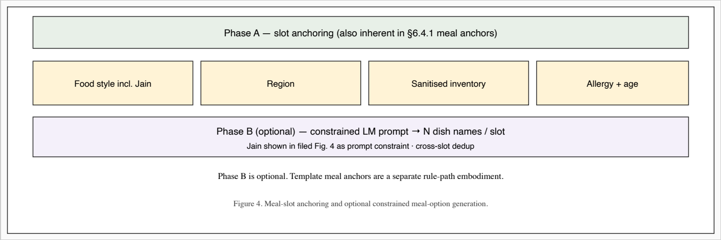
Figure 4 — Meal-slot anchoring and optional constrained meal-option generation.
