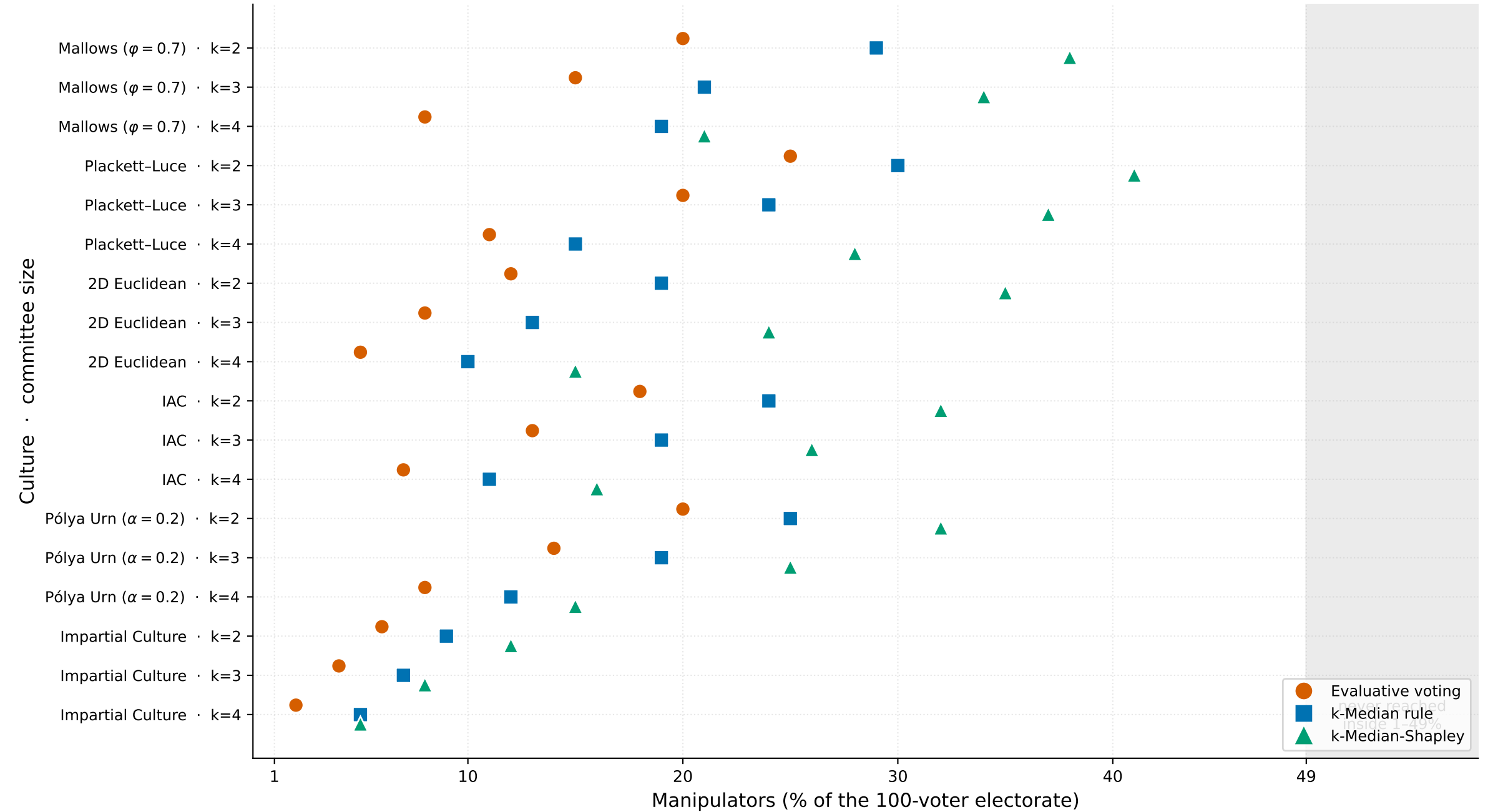
How much manipulation does it take to elect the bottom candidate? Population level (% of the electorate) at which the bottom target reaches a 50% success rate · n = 100 voters, m = 5 candidates, k = 2, 3, 4
