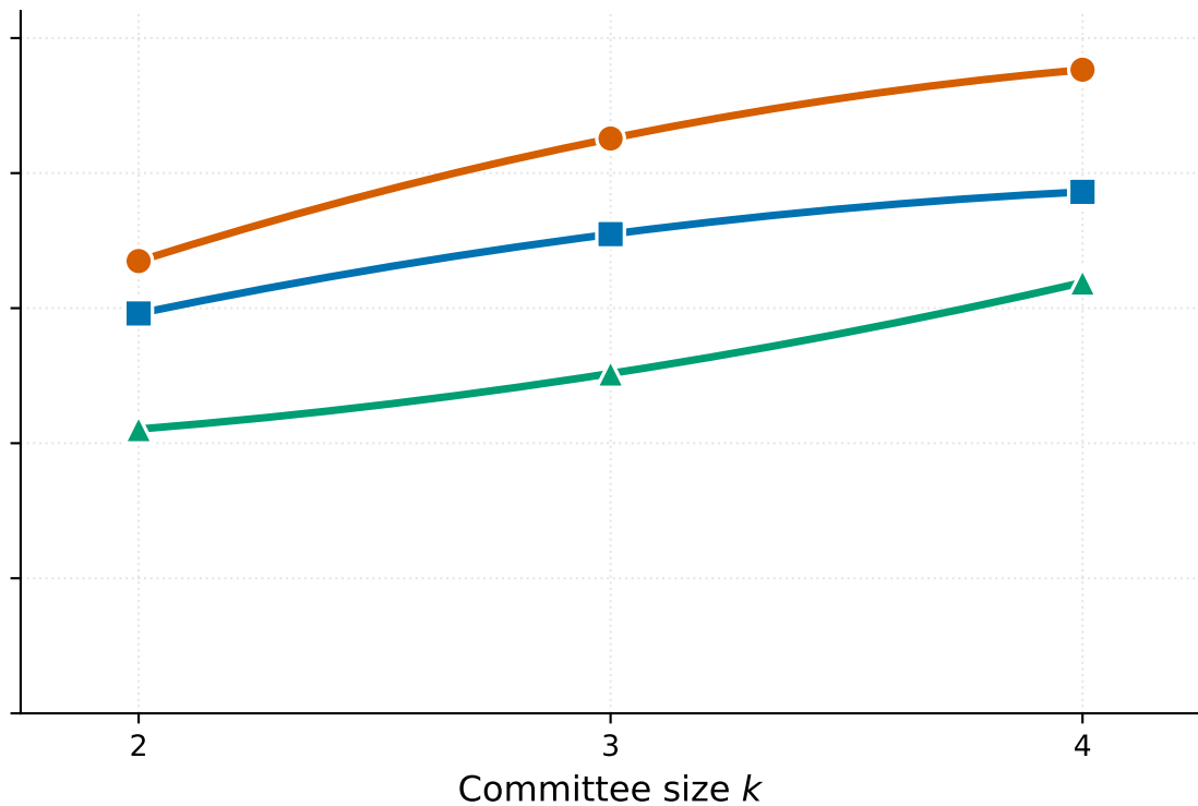
Bottom attack
