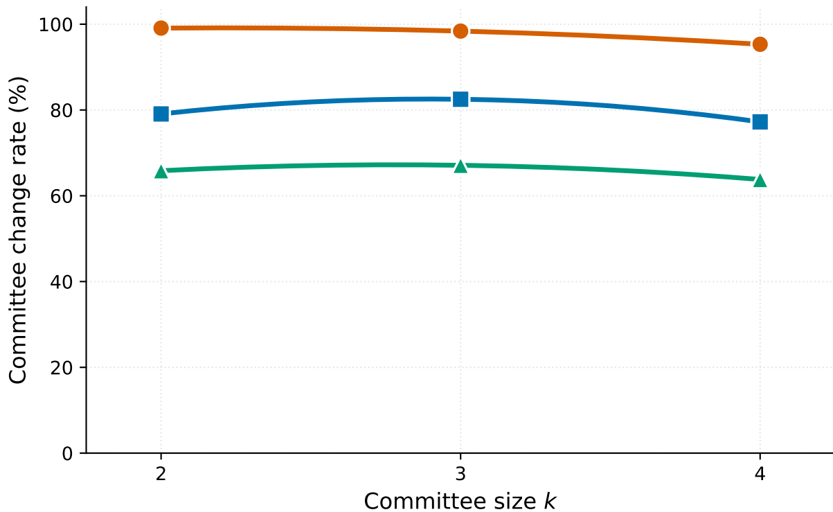
Cutoff attack
