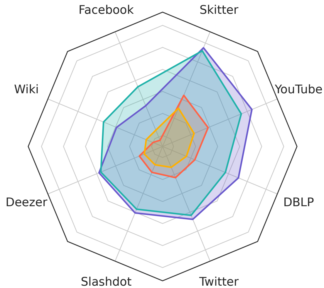
Maximum Coverage
