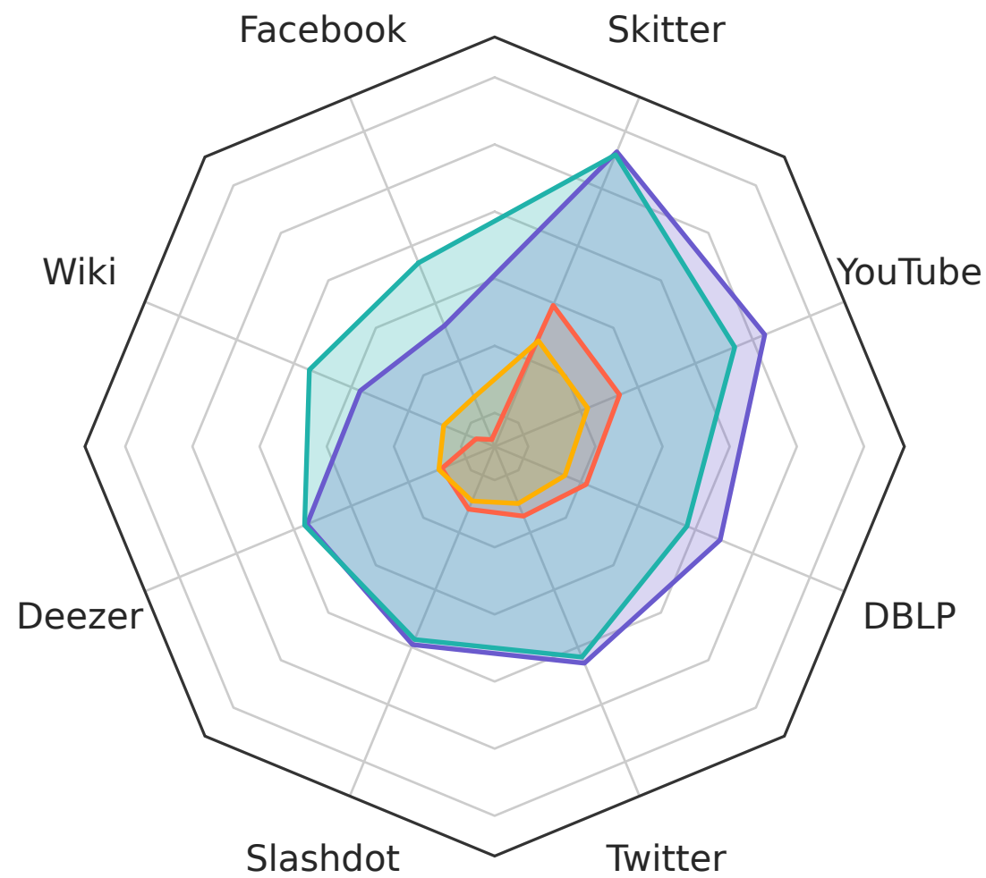
Maximum Cut
