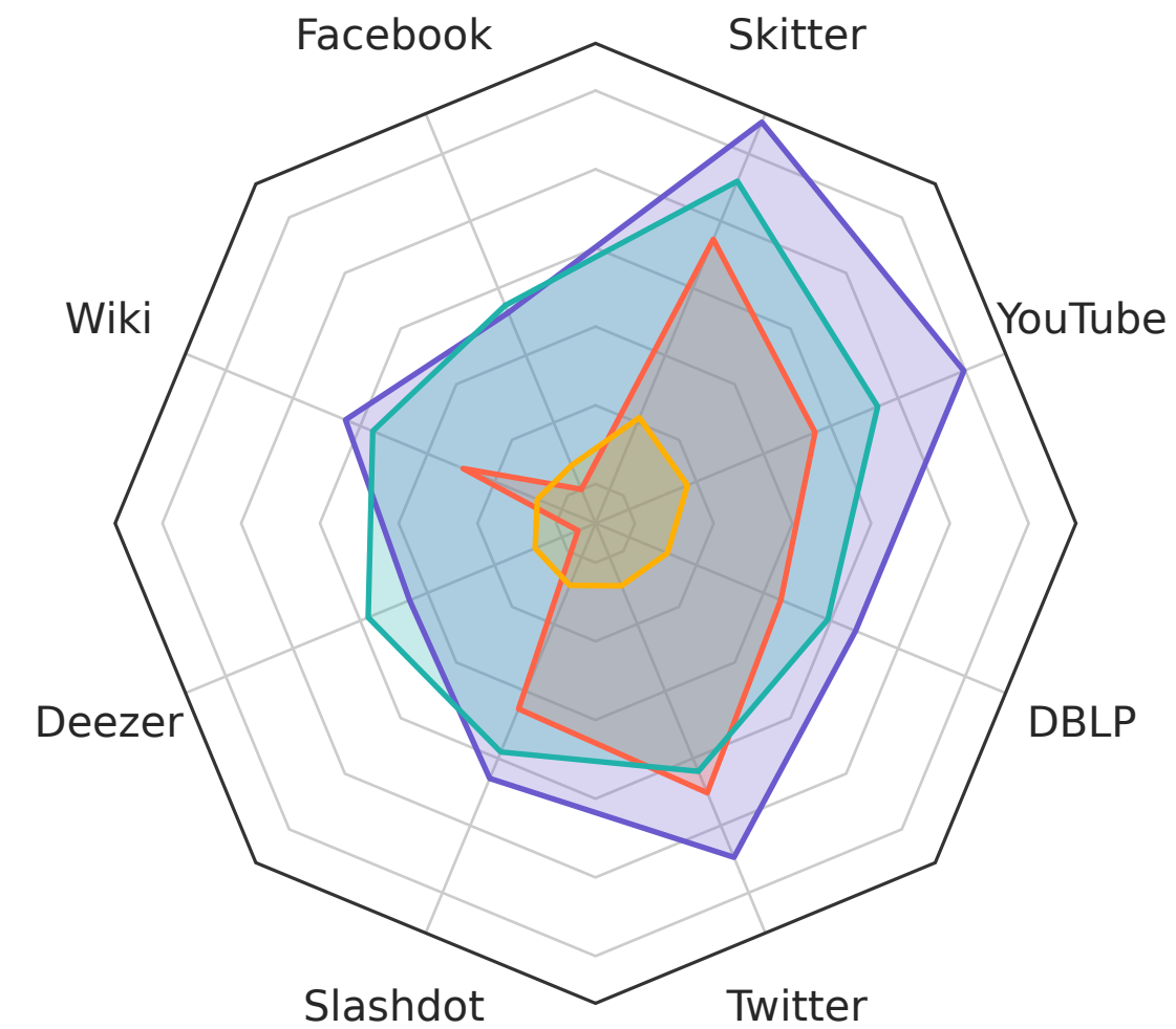
Influence Maximization
