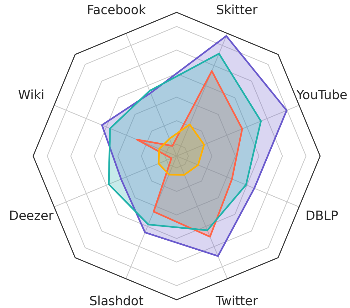
Influence Maximization
