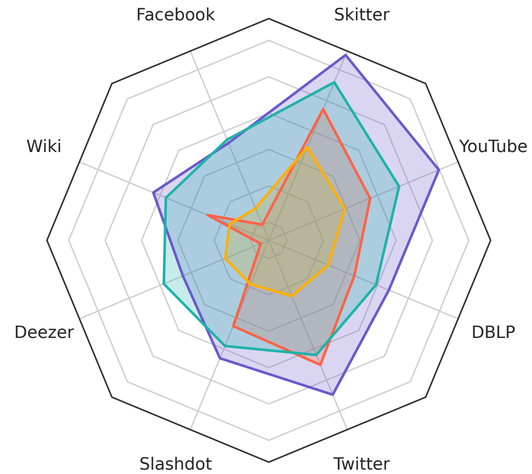
Influence Maximization
