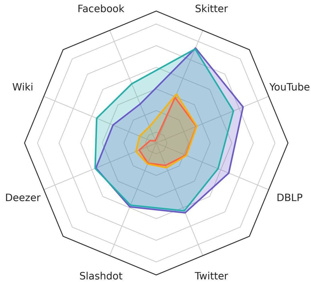
Maximum Cut
