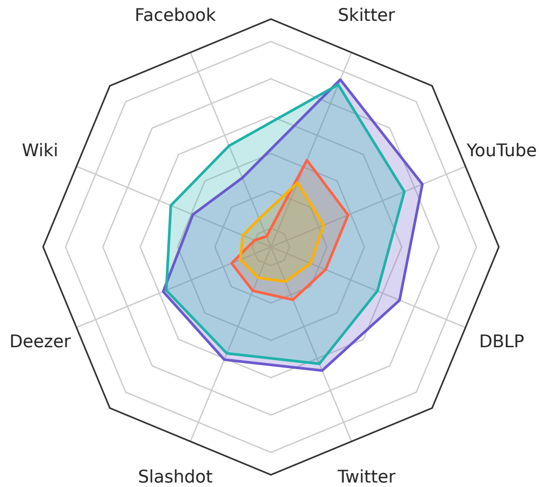
Maximum Coverage
