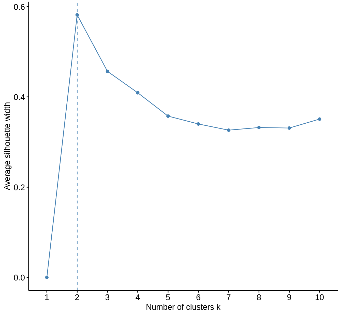
Optimal number of clusters Average silhouette width (scaled iris)
