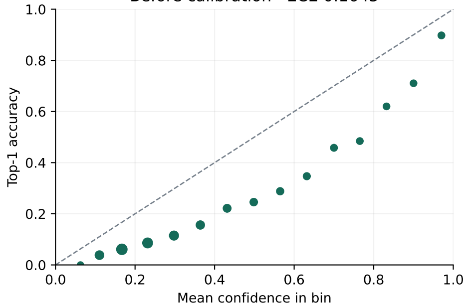
Before calibration · ECE 0.1645
