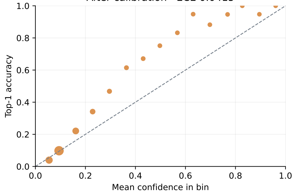
After calibration · ECE 0.0415
