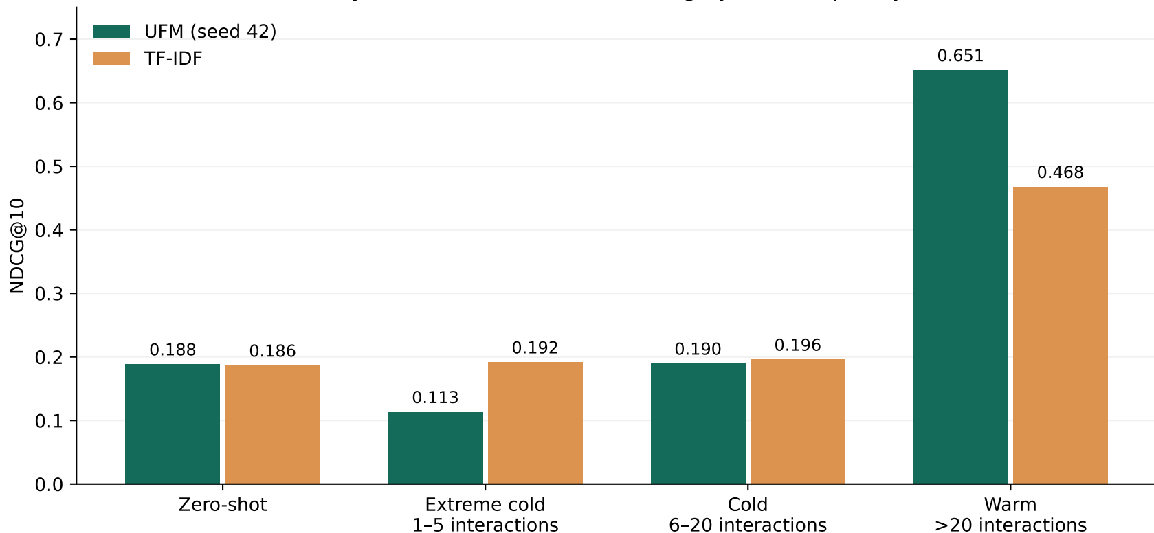
Toys & Games: validation ranking by item frequency
