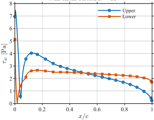
Wall shear stress, \alpha = 10^\circ
