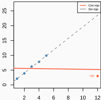
B: Leverage alto, Cook alto
