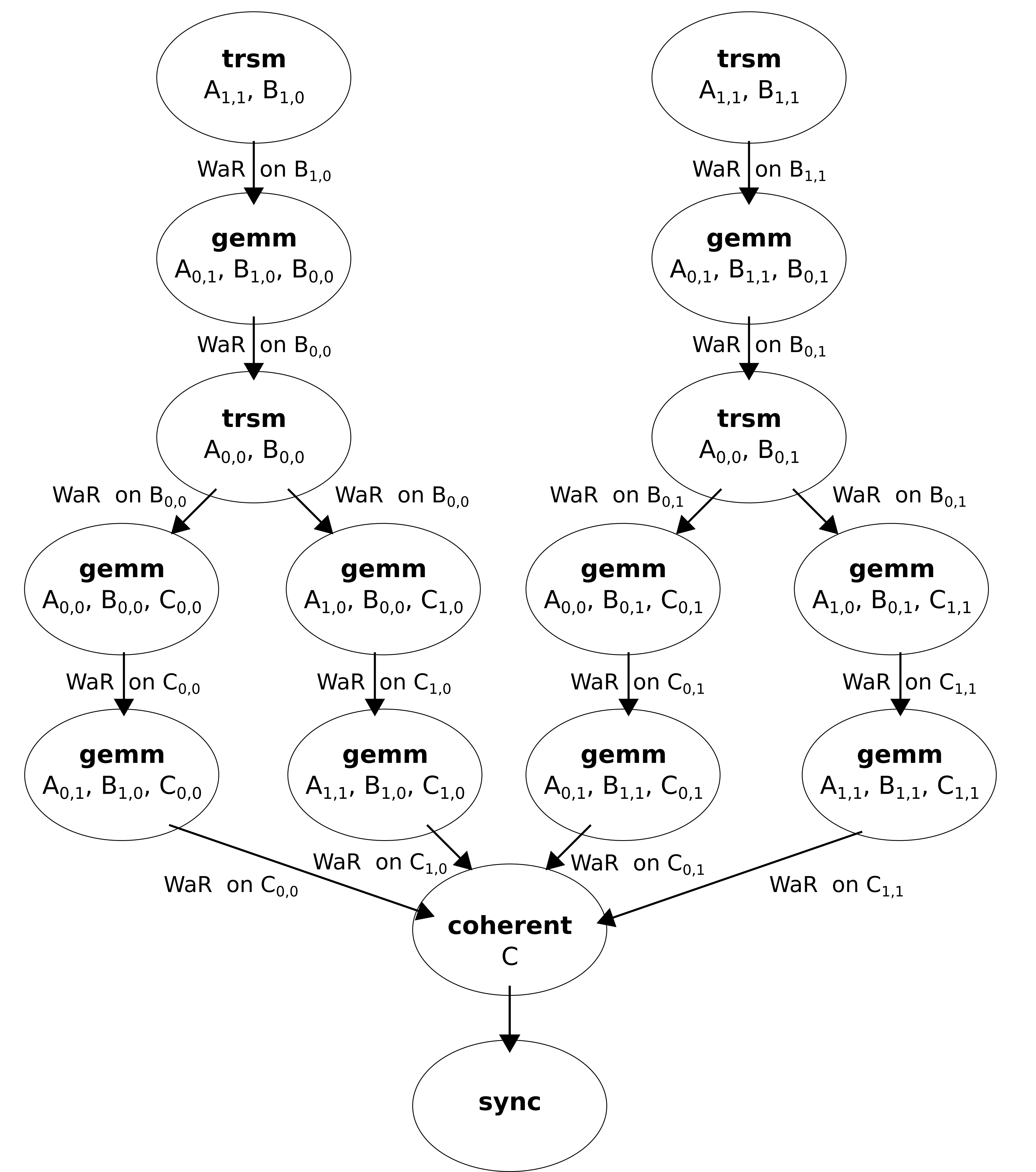
Generated task graph
