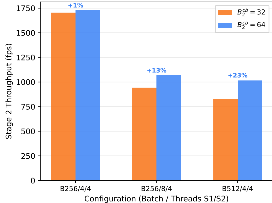
Stage 2 Throughput
