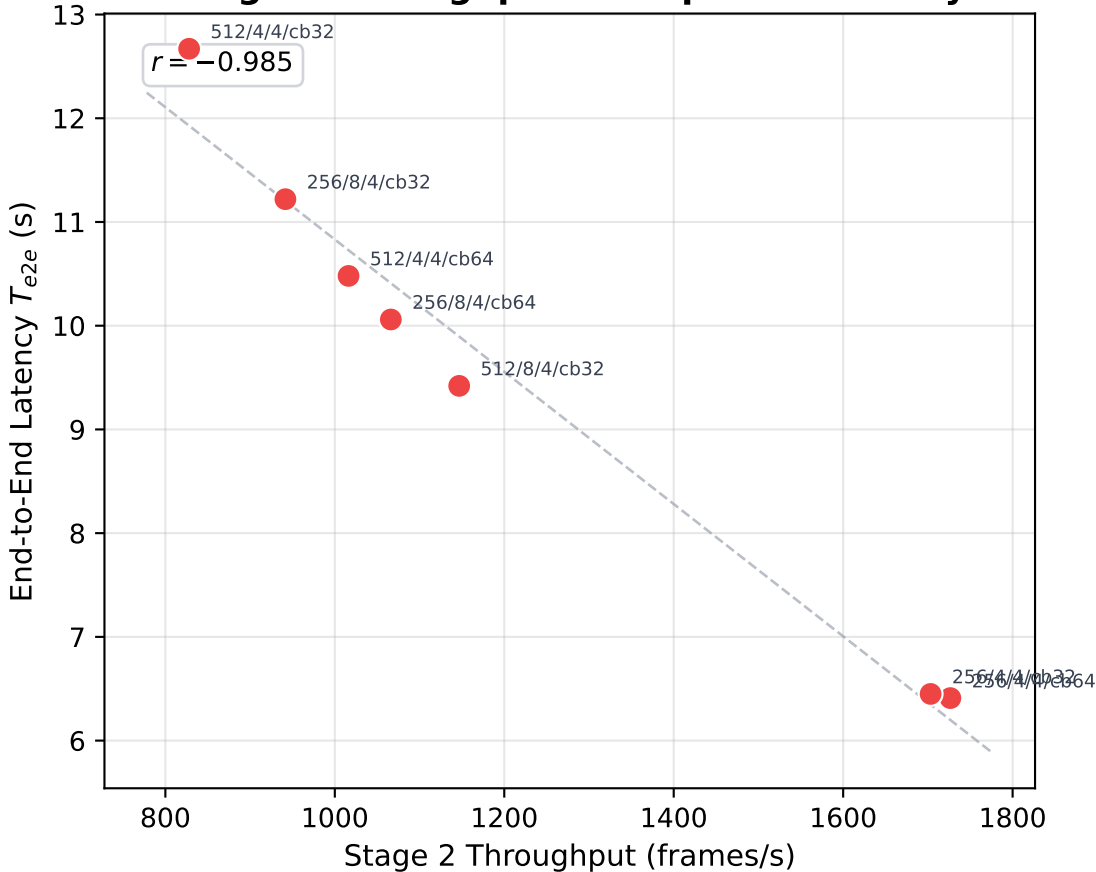
Stage 2 Throughput vs. Pipeline Latency
