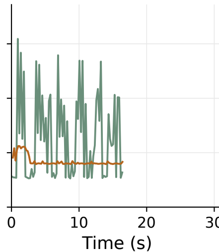
batch 8
