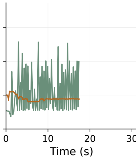
batch 4
