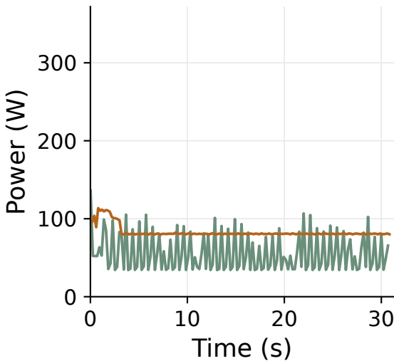
batch 2
