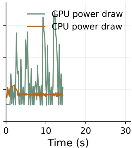
batch 16
