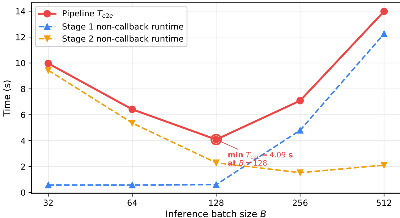
Pipeline latency tracks summed runtime overhead
