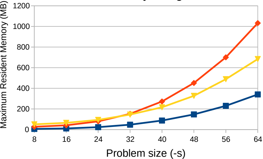
Memory usage
