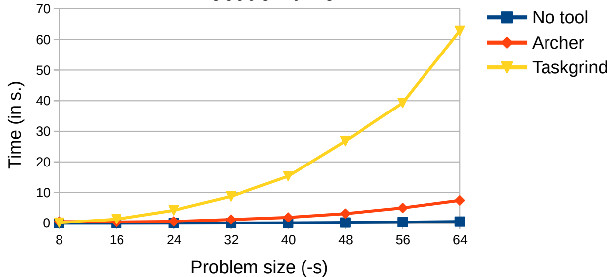
Execution time
