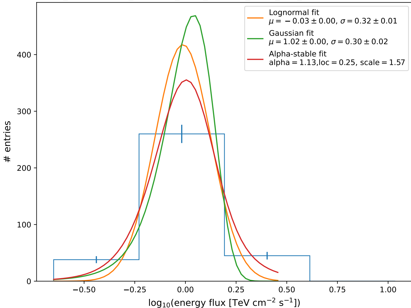
4FGL_J0141.4-0928_FermiLAT_norm_lognorm_alpha_upd_1000 - CTAO simulation
