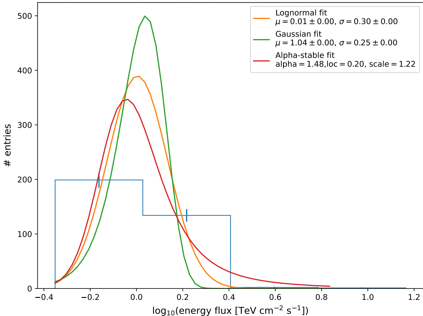
4FGL_J0638.6+7320_FermiLAT_norm_lognorm_alpha_upd_1000 - CTAO simulation
