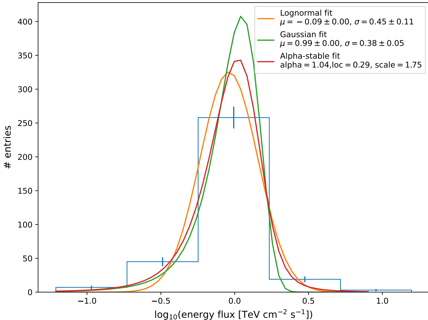
4FGL_J0742.6+5443_FermiLAT_norm_lognorm_alpha_upd_1000 - CTAO simulation
