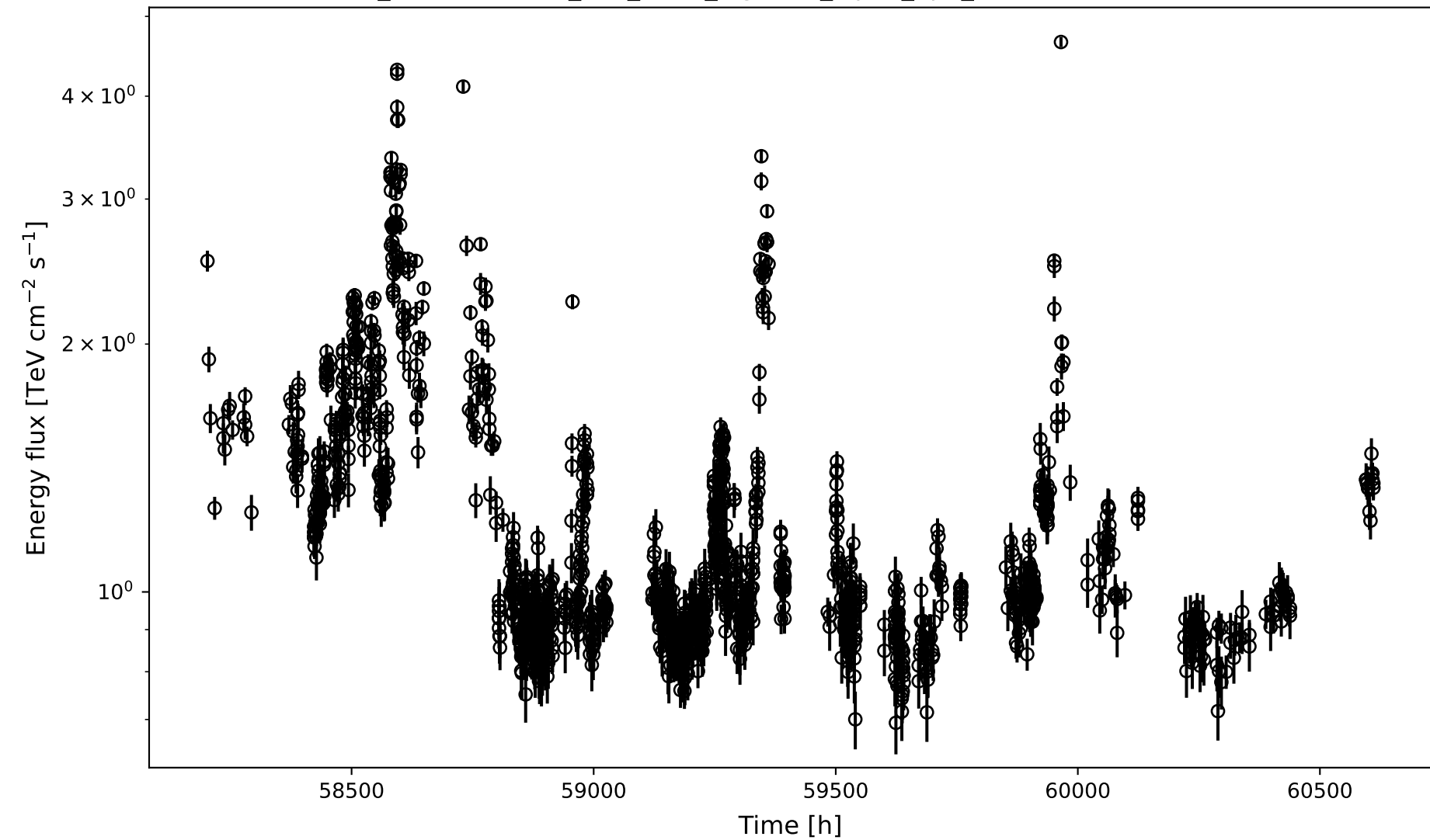
4FGL_J0921.6+6216_ZTF_norm_lognorm_alpha_upd_1000 - CTAO simulation
