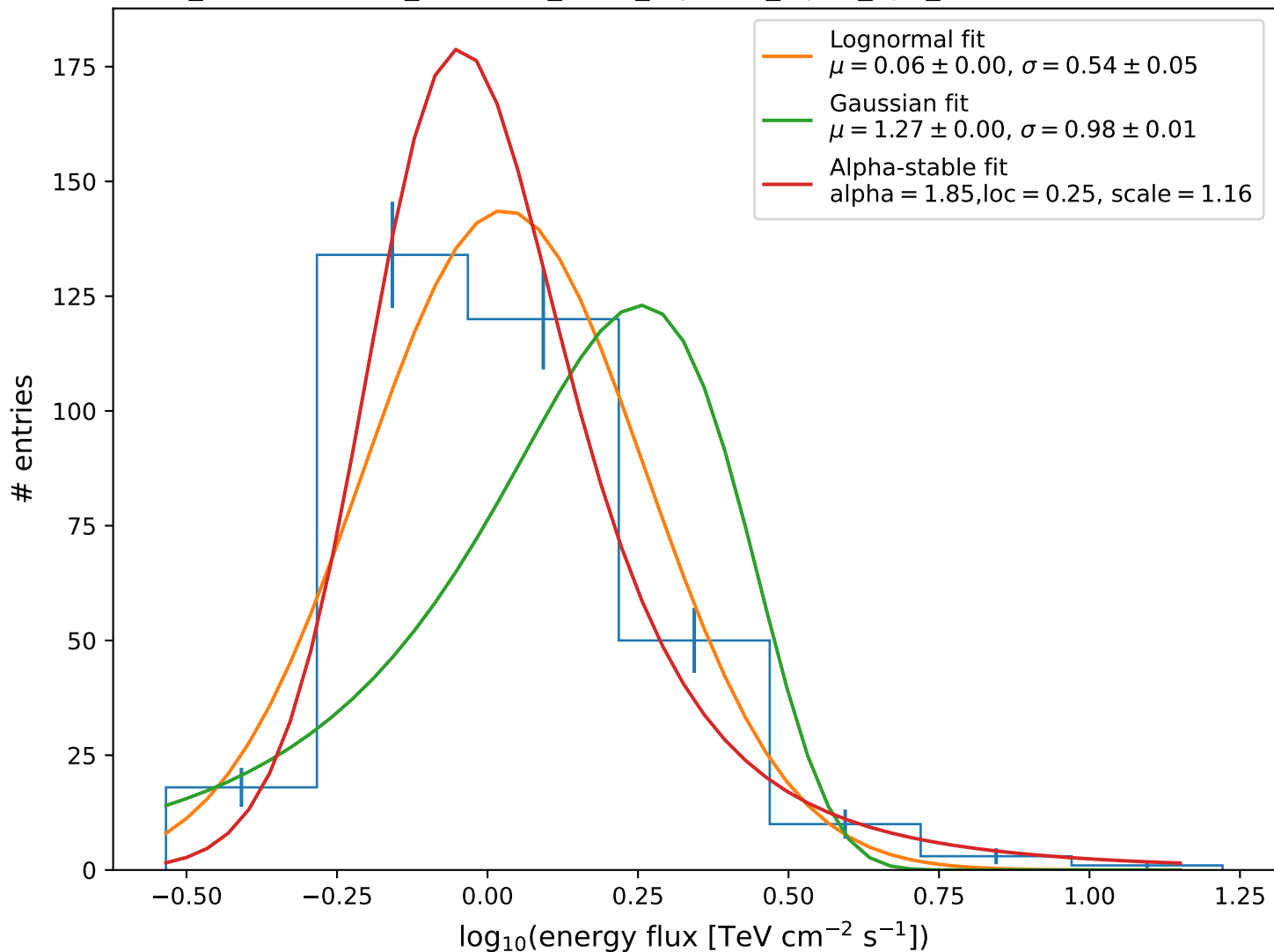
4FGL_J1800.6+7828_FermiLAT_norm_lognorm_alpha_upd_1000 - CTAO simulation
