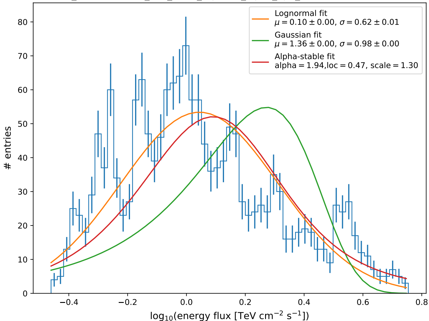
4FGL_J1800.6+7828_ZTF_norm_lognorm_alpha_upd_1000 - CTAO simulation
