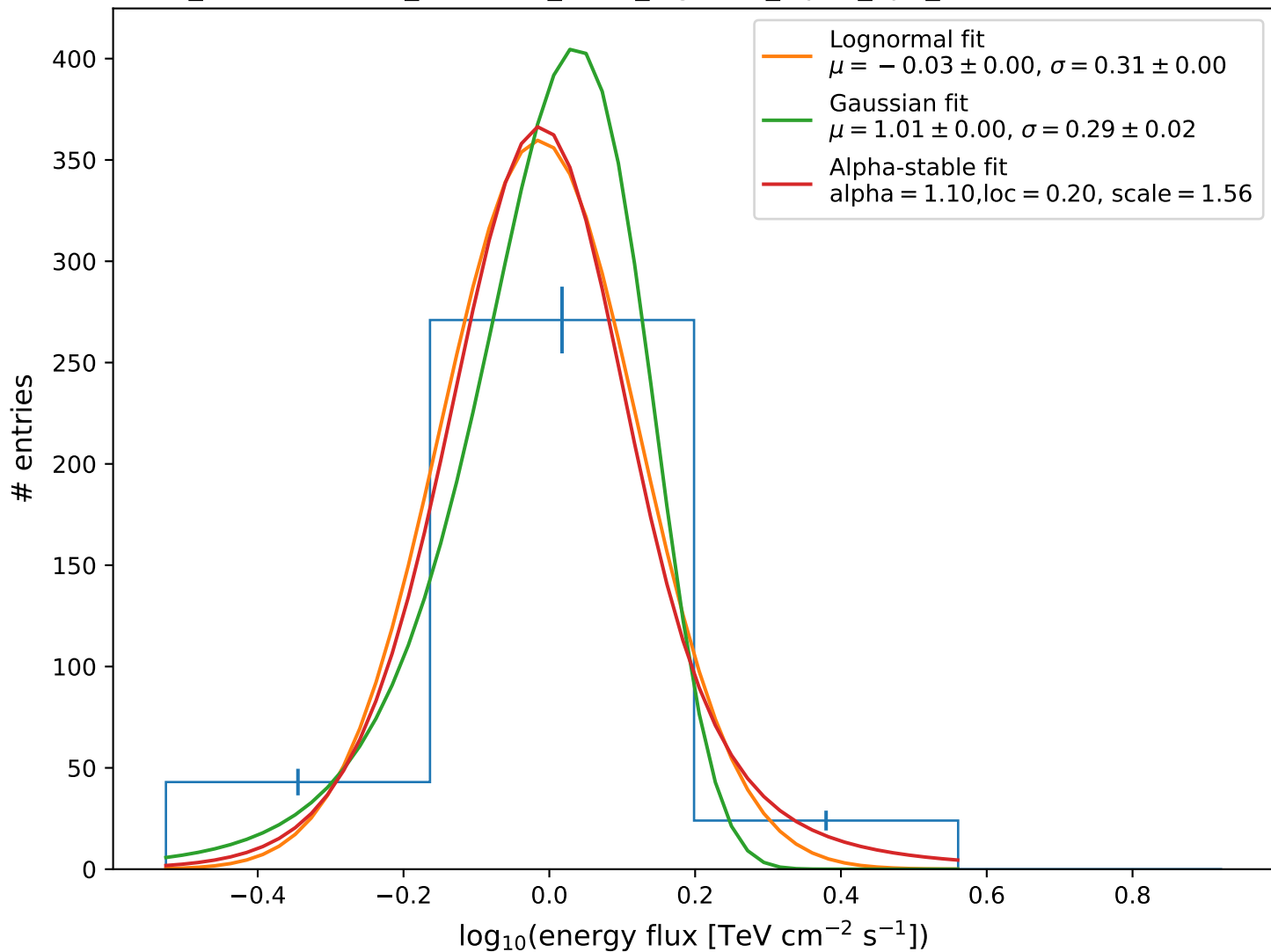
4FGL_J1813.5+3144_FermiLAT_norm_lognorm_alpha_upd_1000 - CTAO simulation
