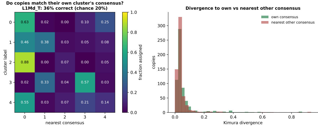
Figure 12: Cross-check of the clusters against the consensus alignments for L1Md_T . Left: fraction of each cluster's copies whose nearest consensus is each cluster's, after projecting every copy onto every consensus with mafft -addfragments -keeplength . A subfamily assignment would put the mass on the diagonal; the observed 36.1% (chance 20.0%) does not. Right: Kimura divergence of each copy to its own cluster's consensus versus to the nearest other consensus; the distributions overlap, with the median copy marginally closer to another cluster's consensus.
