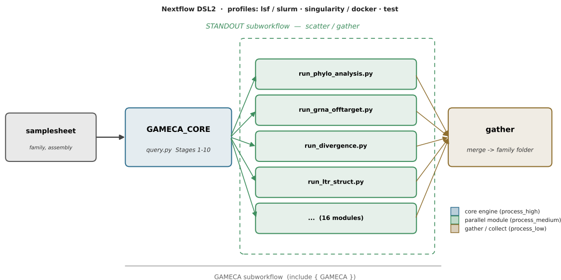
Figure 15: The Nextflow DSL2 execution graph: the core engine feeds a scatter of independent copy-resolved module tasks, gathered into a single per-family output. Profiles select LSF or Slurm and Singularity or Docker.
