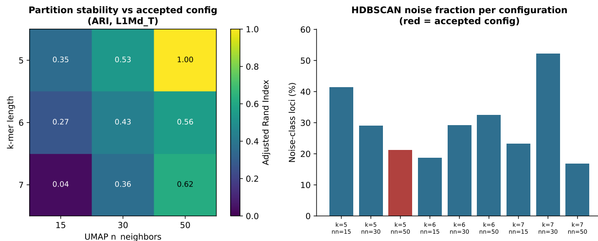
Figure 12: Clustering and noise-class validation for L1Md_T . Left: Adjusted Rand Index of each k and n\_neighbors configuration against the configuration the automatic search accepted. Values near 1 would indicate the partition is independent of the parameter choice; the observed median of 0.40 indicates it is not, which is why these sub-family boundaries are not interpreted as biological. Right: HDBSCAN noise-class fraction per configuration, with the accepted configuration highlighted. Noise-class loci are retained as a labelled group and excluded from consensus building.
