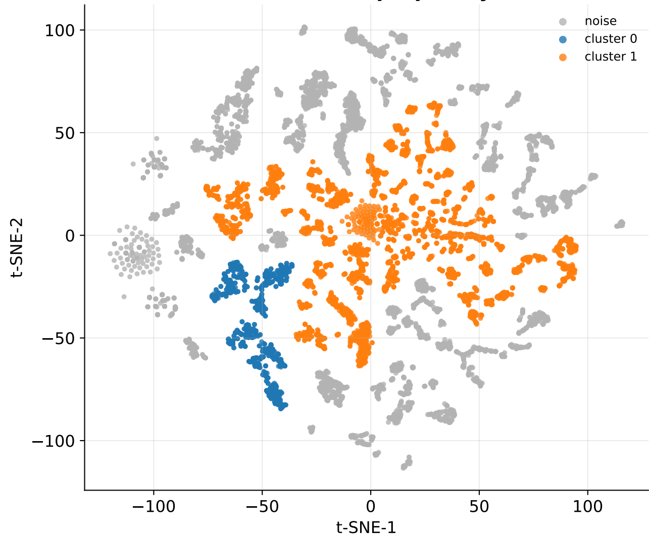
IAP — 2D t-SNE (perplexity=30)
