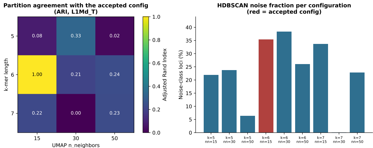
Figure 11: Clustering and noise-class validation for L1Md_T . Left: Adjusted Rand Index of each k and n\_neighbors configuration against the configuration the automatic search accepted. Values near 1 would indicate the partition is independent of the parameter choice; the observed median of 0.21 indicates it is not, which is why these sub-family boundaries are not interpreted as biological. Right: HDBSCAN noise-class fraction per configuration, with the accepted configuration highlighted. Noise-class loci are retained as a labelled group and excluded from consensus building.
