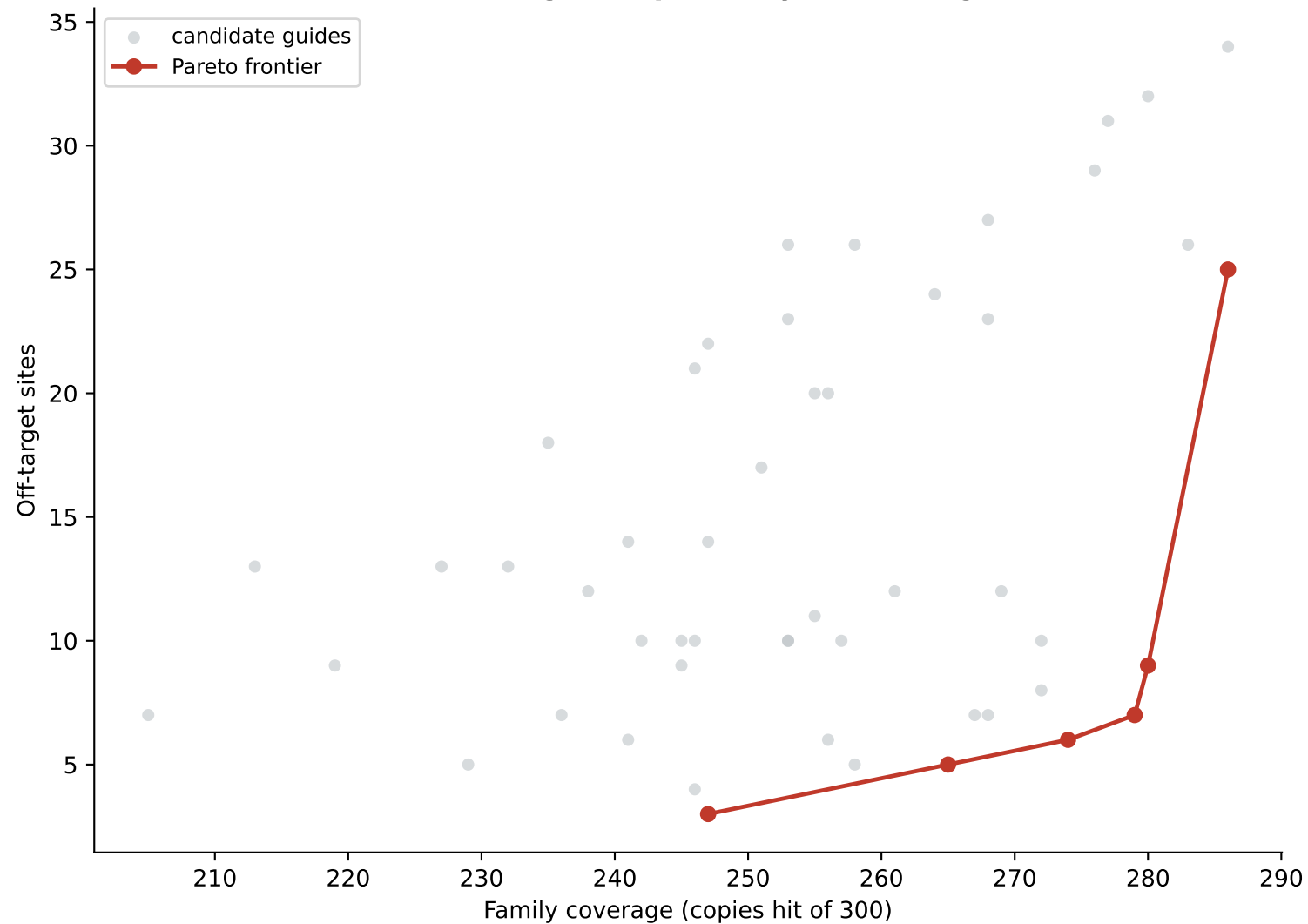
AluYa5 --- gRNA specificity vs coverage
