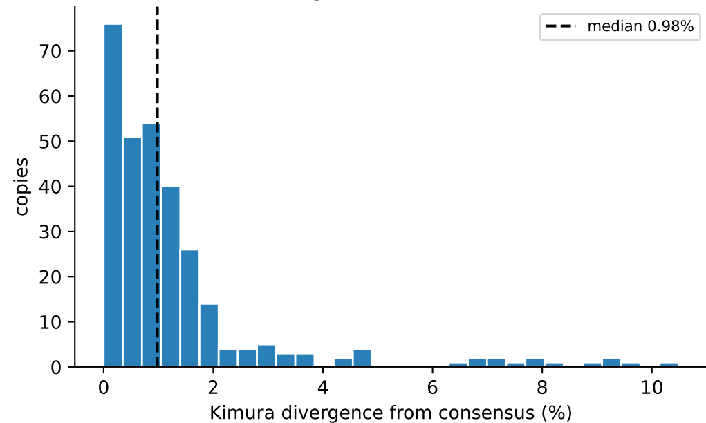
Divergence distribution
