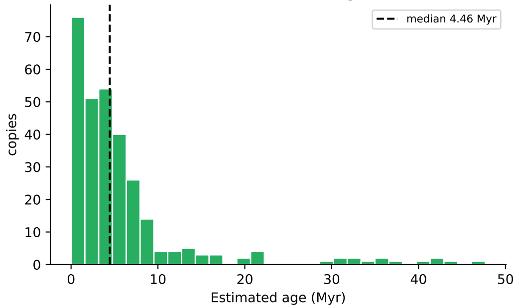
Molecular-clock age
