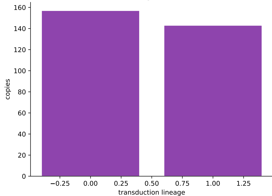
Lineage sizes
