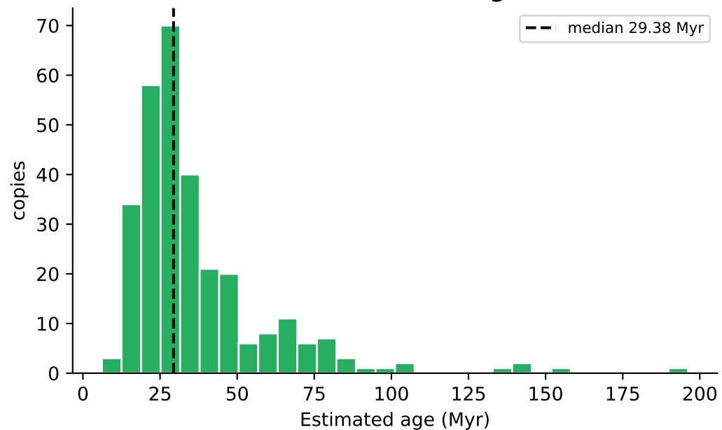
Molecular-clock age
