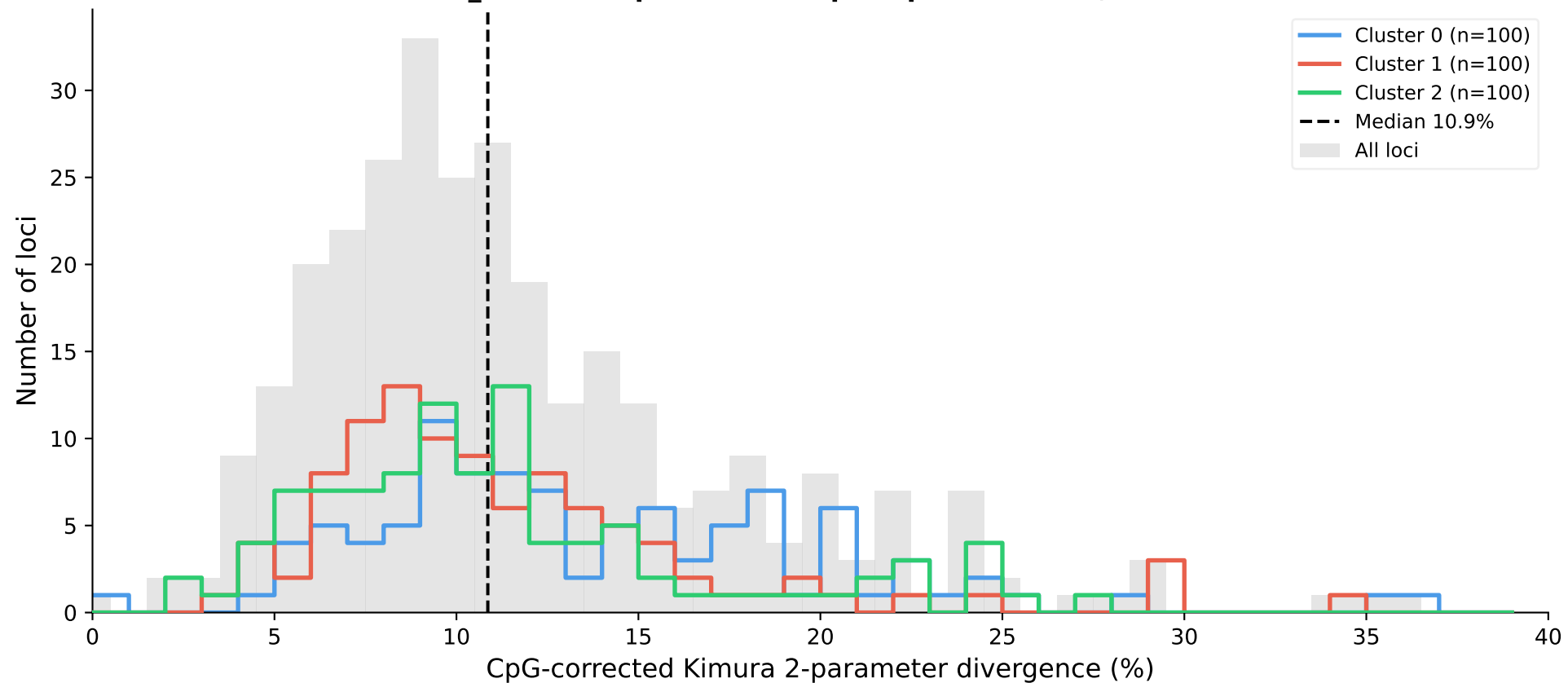
B2_Mm2 — Repeat Landscape (CpG-corrected, \omega=10 )
