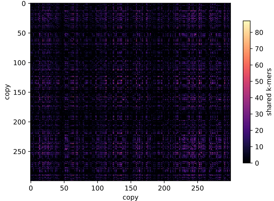
Shared transduced k-mers
