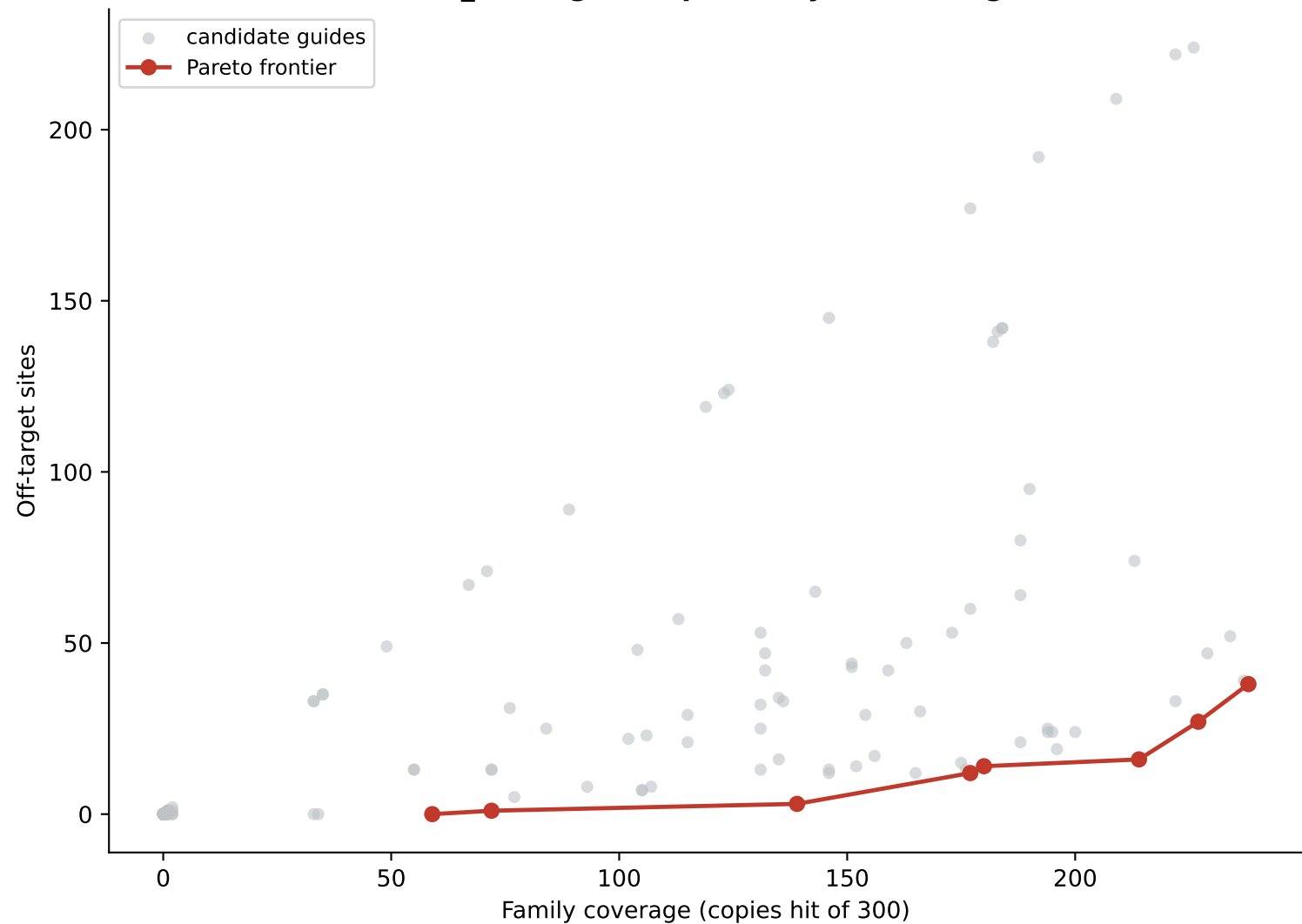
LTR5_Hs --- gRNA specificity vs coverage
