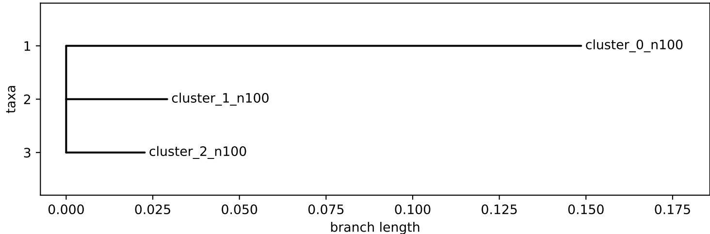
LTR5_Hs --- neighbour-joining tree (3 tips)
