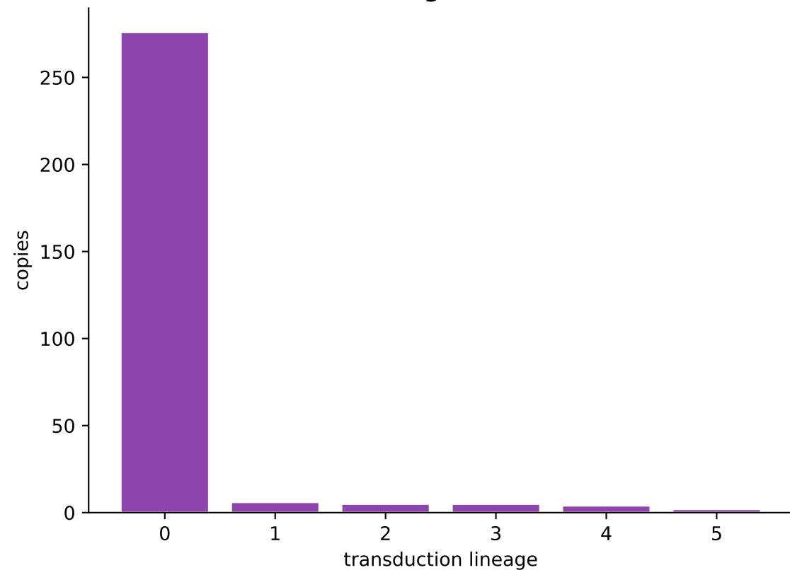
Lineage sizes
