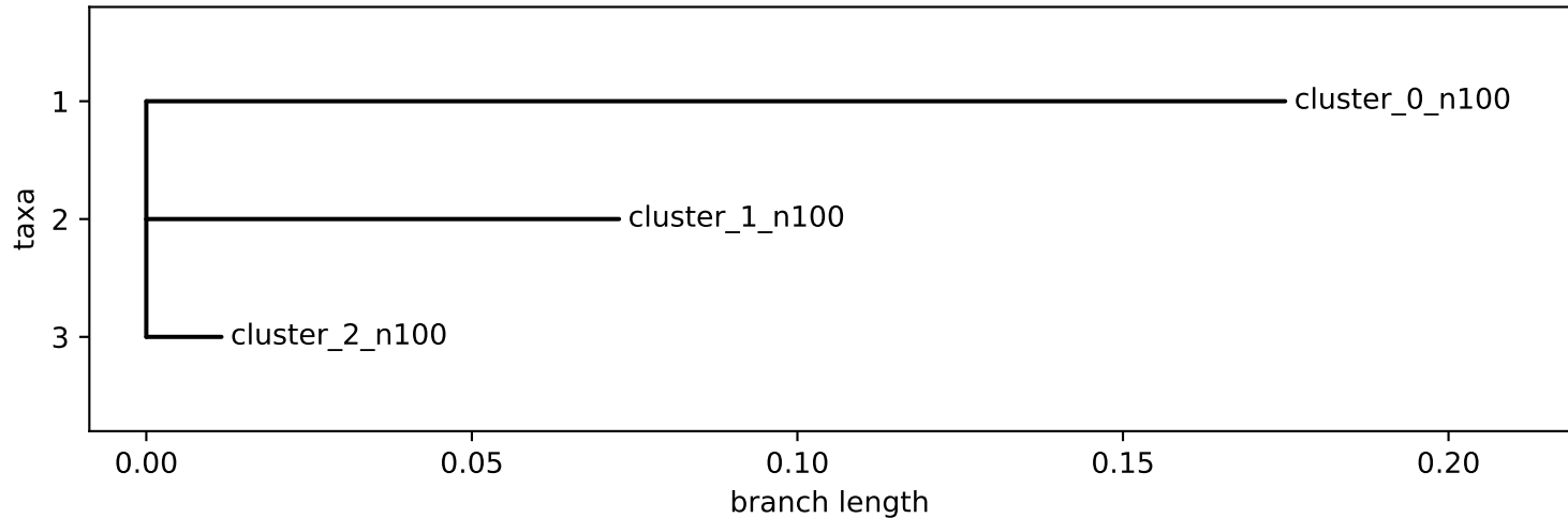
MT2_Mm --- neighbour-joining tree (3 tips)
