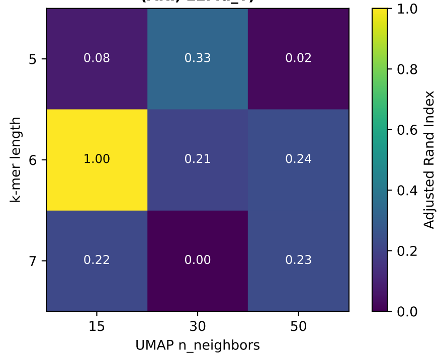
Partition stability vs accepted config (ARI, L1Md_T)
