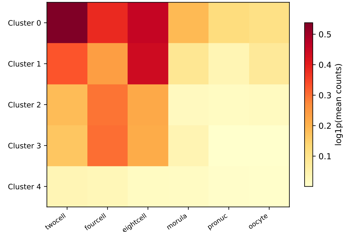
(b) Expression per cluster (log1p mean)
