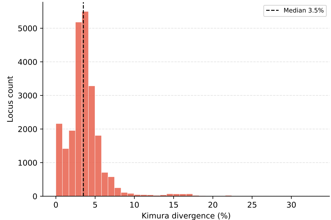
(c) Repeat landscape (LINE)
