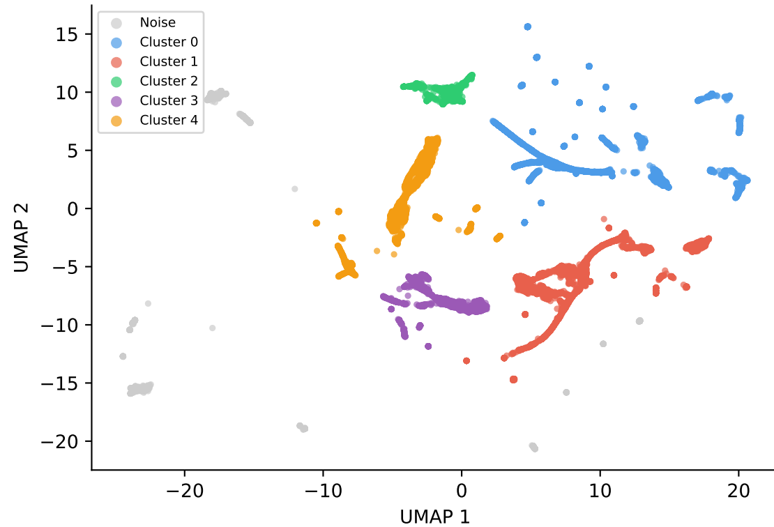
(a) L1Md_T UMAP clustering (5 clusters)
