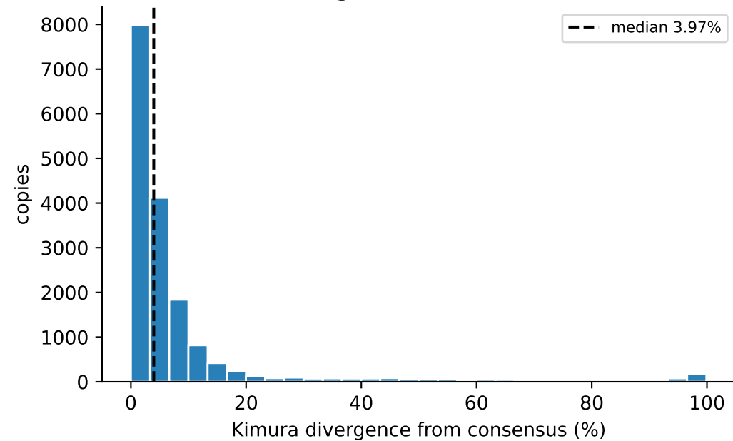
Divergence distribution
