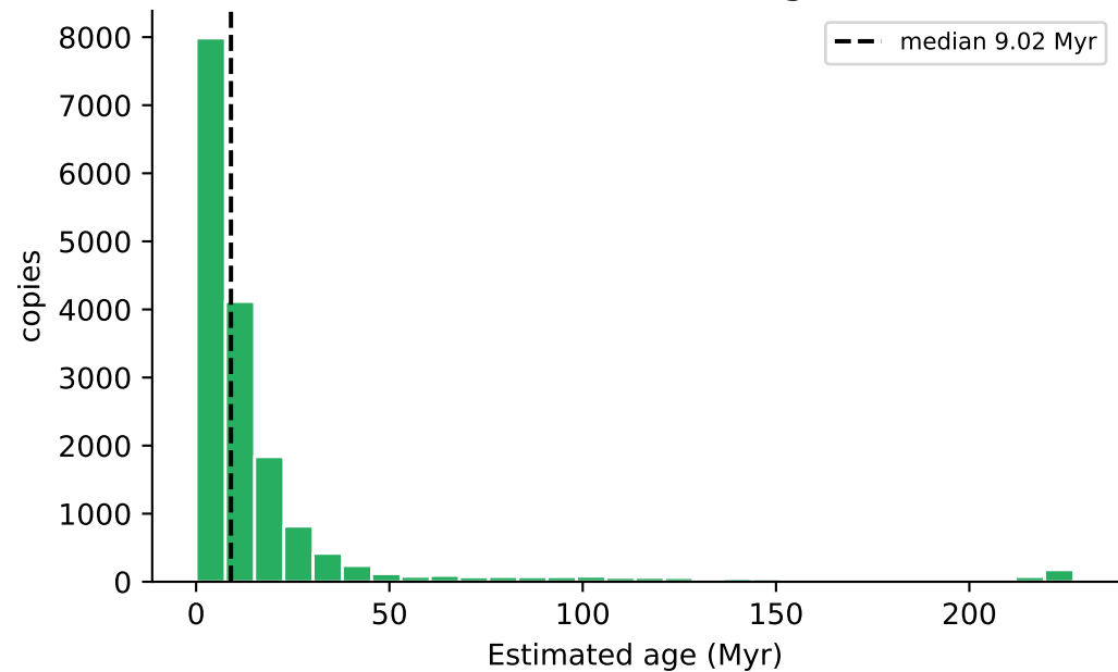
Molecular-clock age
