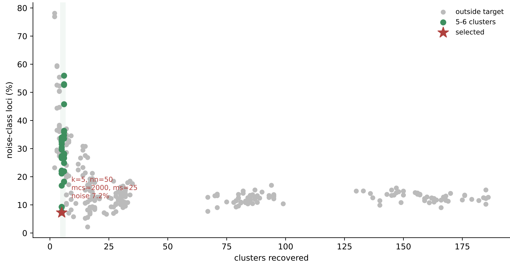
Clustering parameter search: L1Md_T 288 configurations
