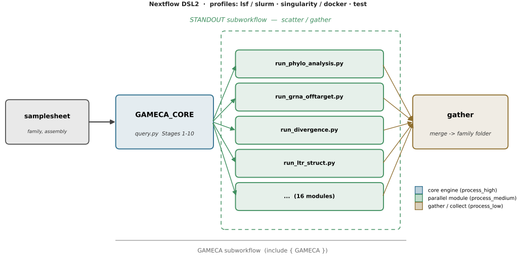
Figure 4: Nextflow DSL2 orchestration. GAMECA_CORE runs query.py Stages 1–10; the STANDOUT subworkflow scatters the copy-resolved analysis modules into independent, individually-resourced GAMECA_STANDOUT tasks that run in parallel and are gathered back per family. The composable GAMECA subworkflow ( CORE → STANDOUT ) is importable into other DSL2 pipelines; execution backend and container runtime are chosen by profile ( lsf/slurm , singularity/docker ).
