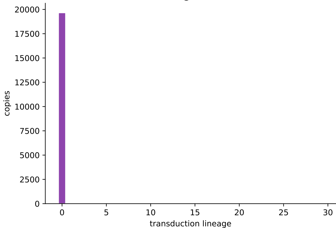
Lineage sizes
