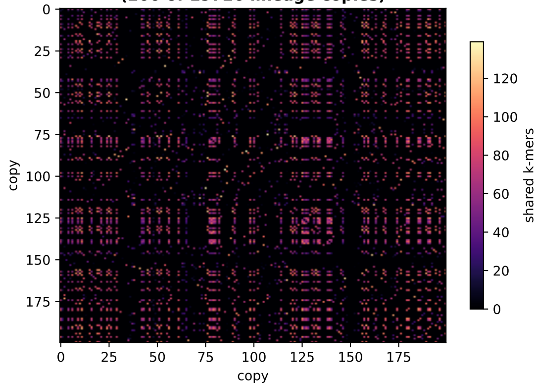
Shared transduced k-mers (200 of 19726 lineage copies)
