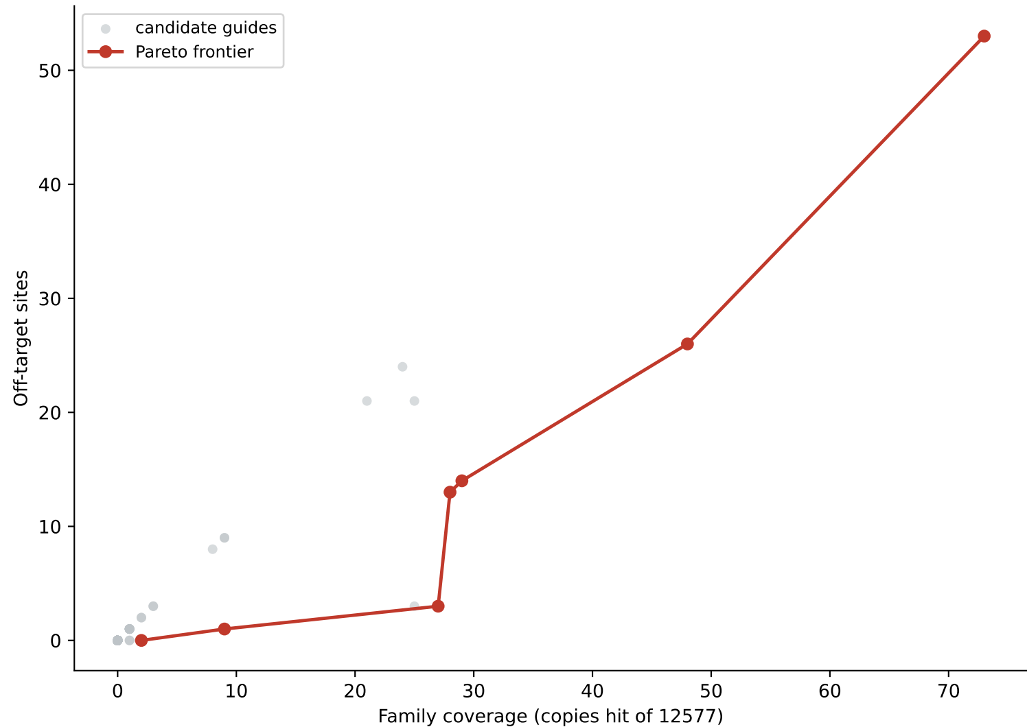
IAP --- gRNA specificity vs coverage
