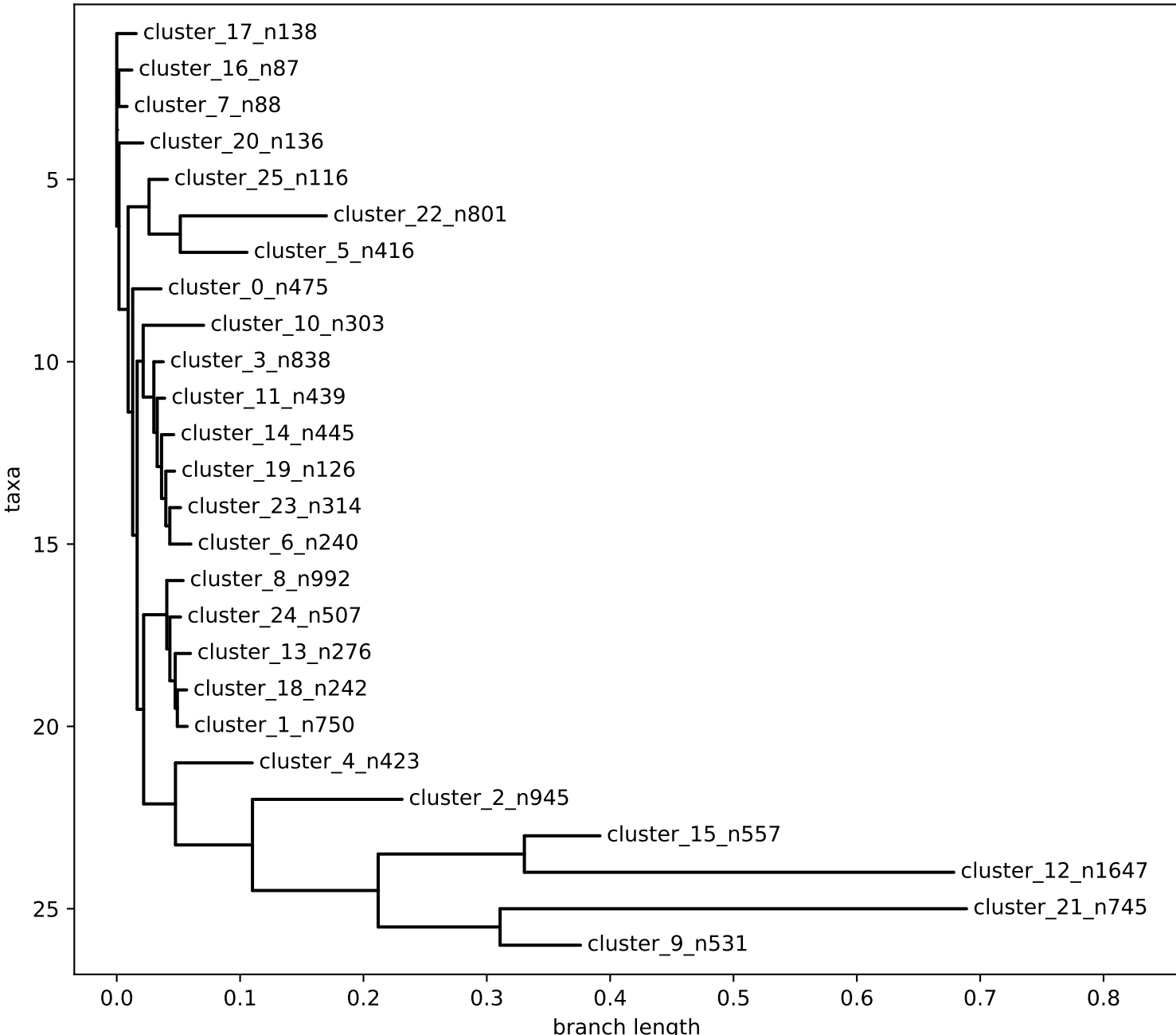
IAP --- neighbour-joining tree (26 tips)
