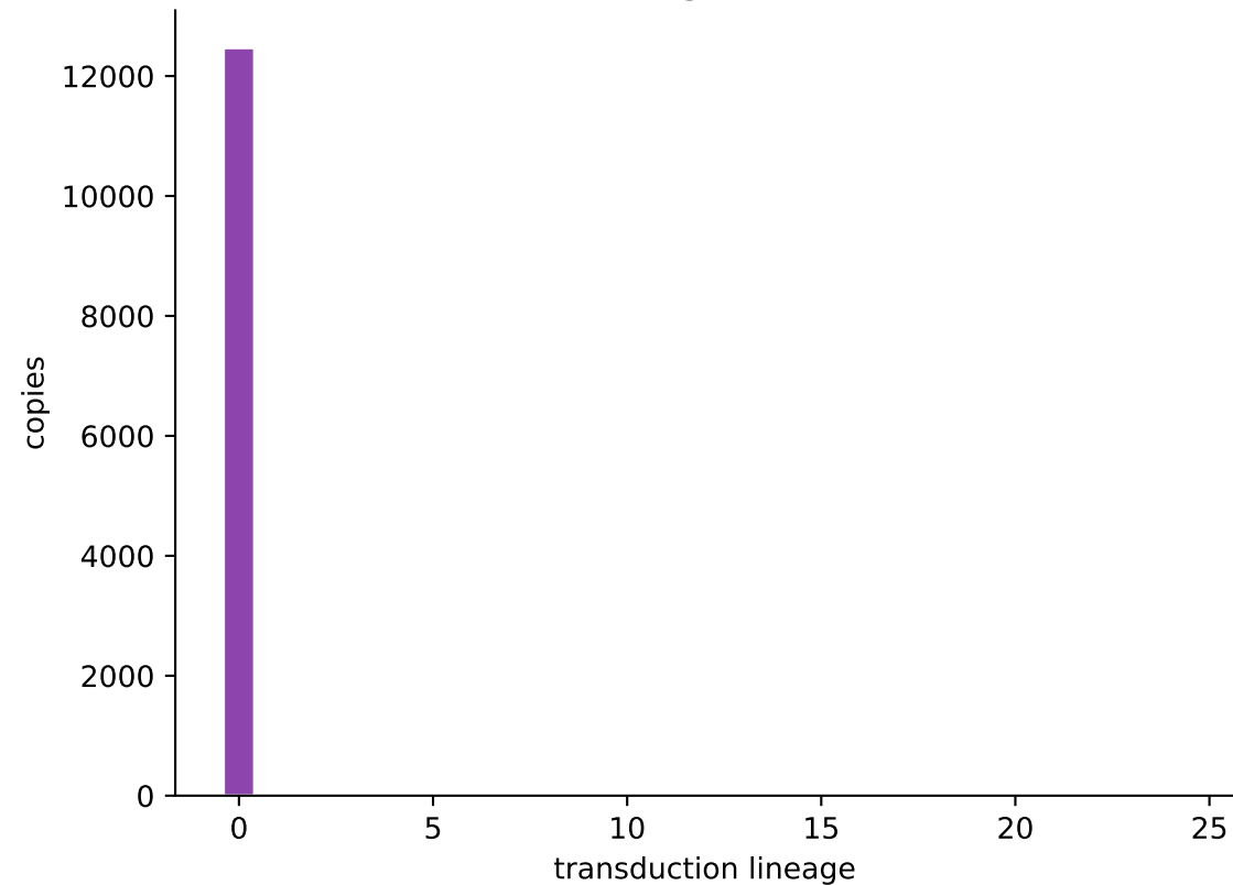
Lineage sizes
