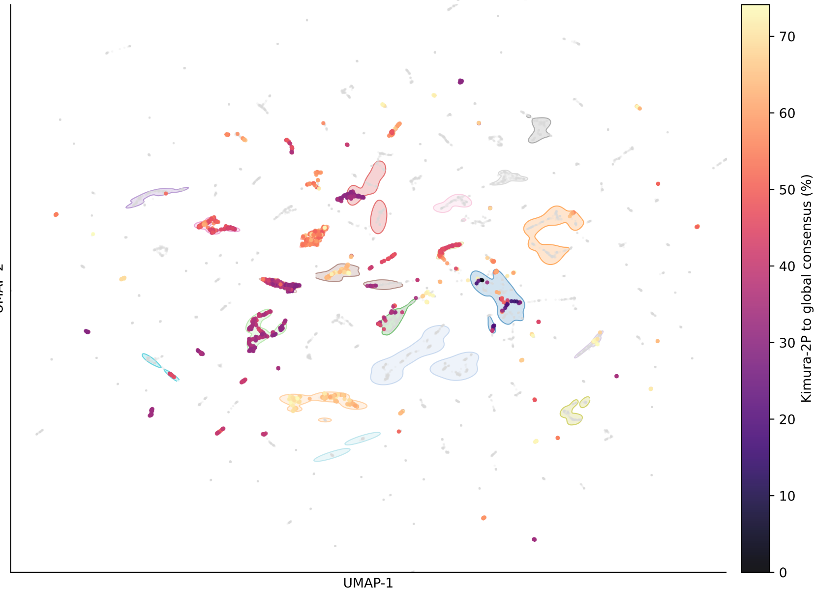
IAP UMAP - distance to global consensus overall mu = 48.9% (N = 2,796 good copies)
