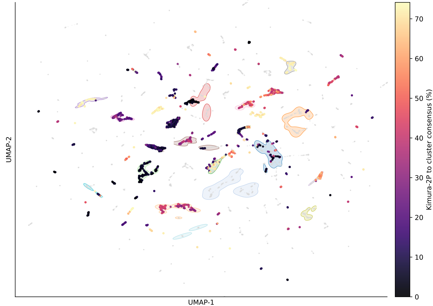
IAP UMAP - distance to cluster consensus overall mu = 29.7% (N = 4,185 good copies)
